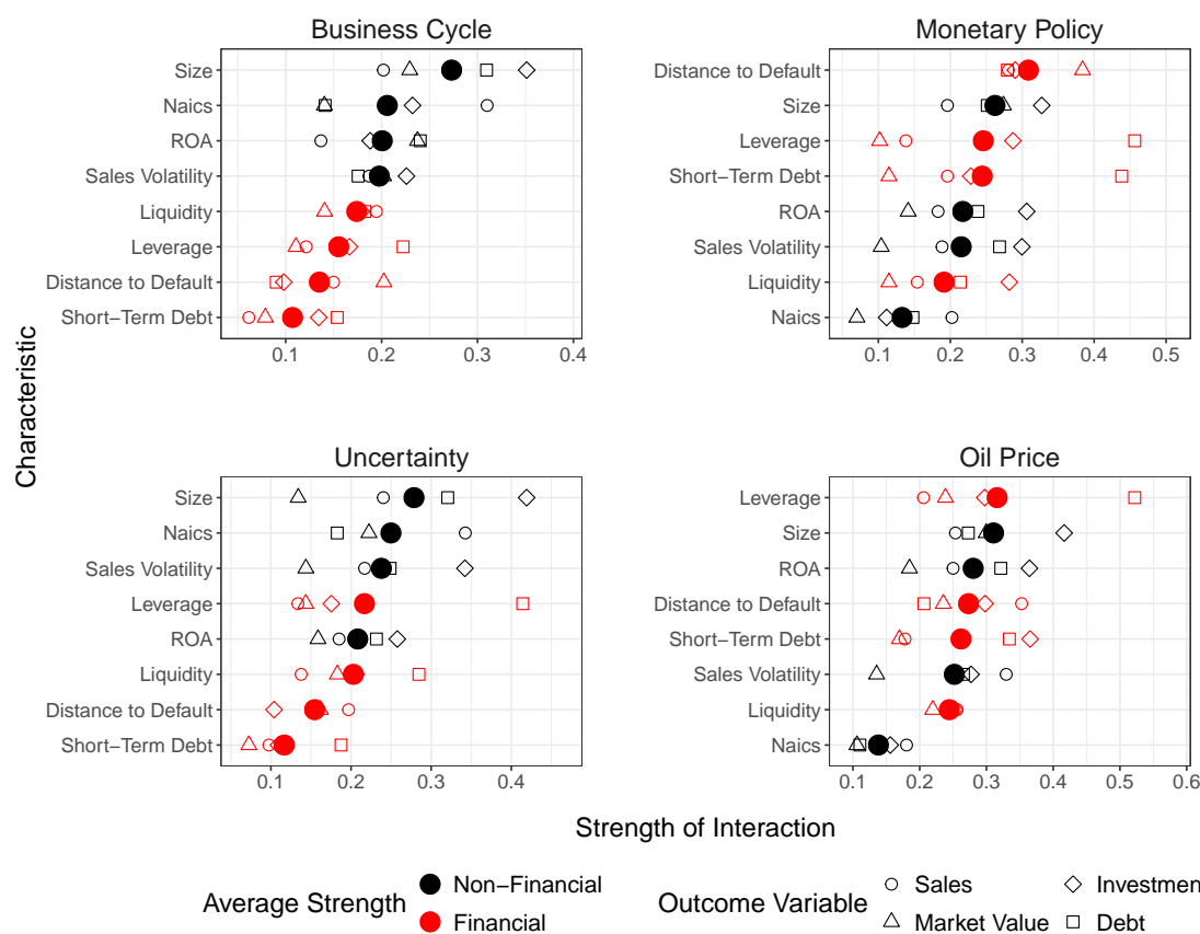
Figure 1: Strength of interactions
