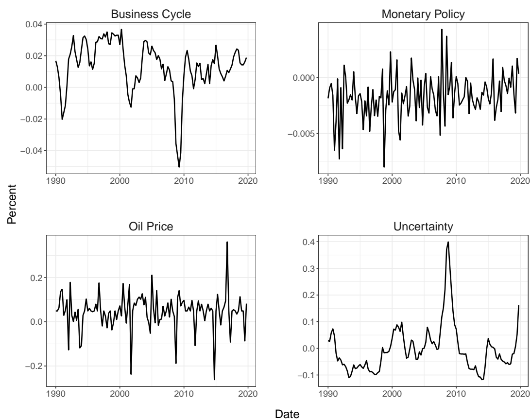
Figure 8: Time series of the aggregate fluctuations
