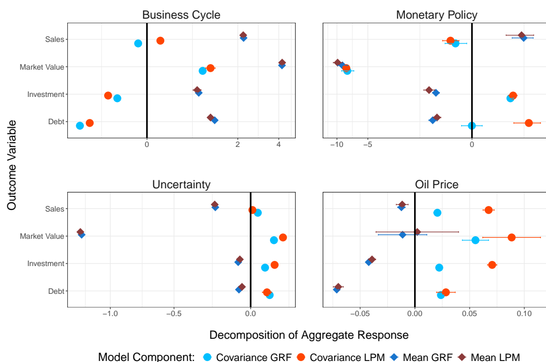
Figure 17: Comparison Mean - Covariance Decomposition
