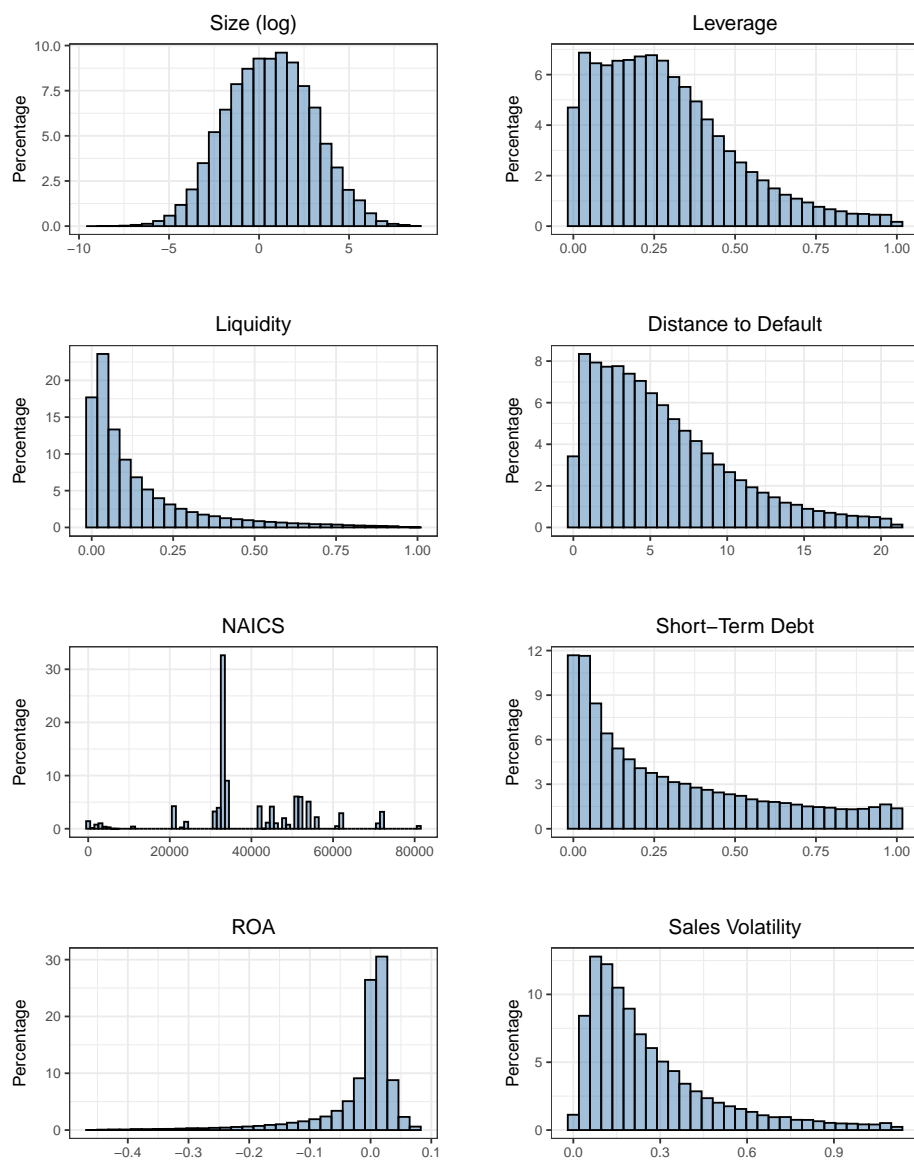
Figure 6: Distribution of the independent variables
