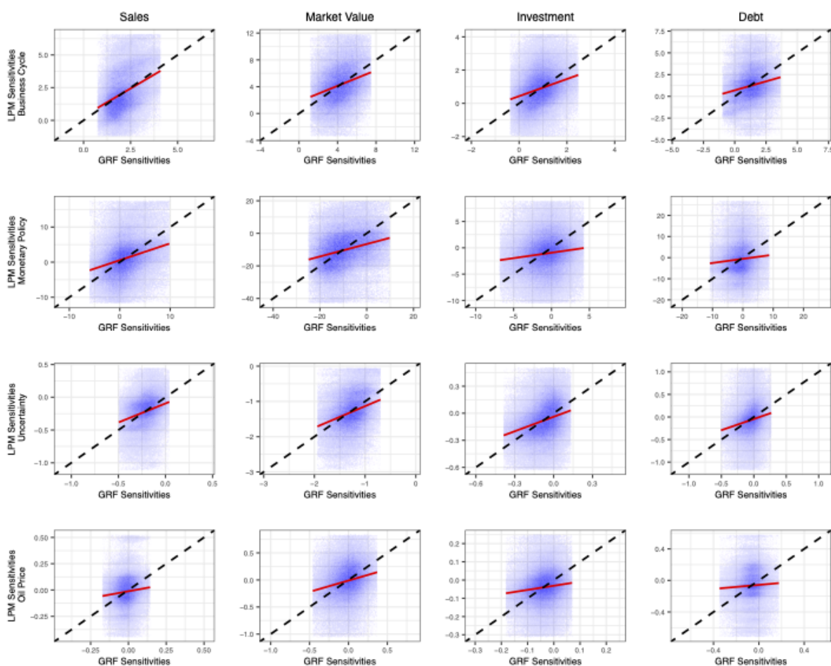
Figure 11: Comparison of sensitivities on actual data
