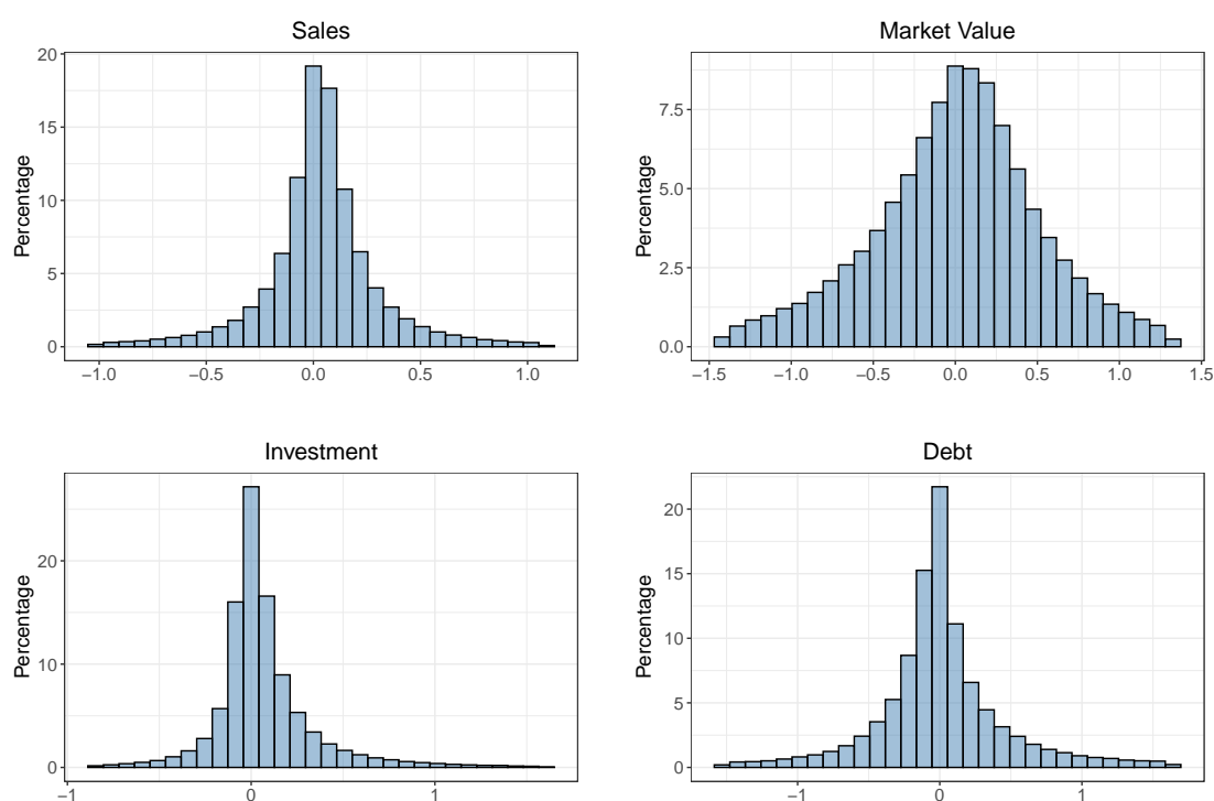
Figure 7: Distribution of the dependent variables
