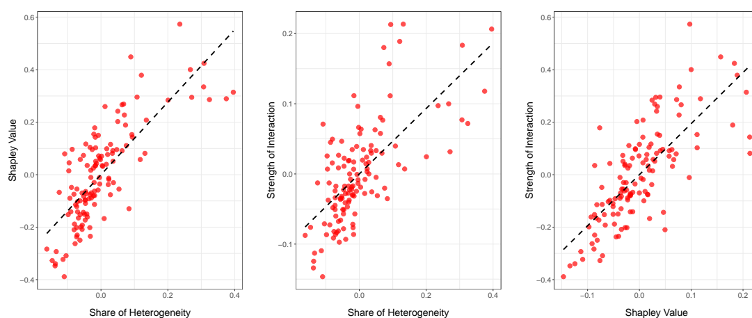
Figure 16: Correlation between importance measures
