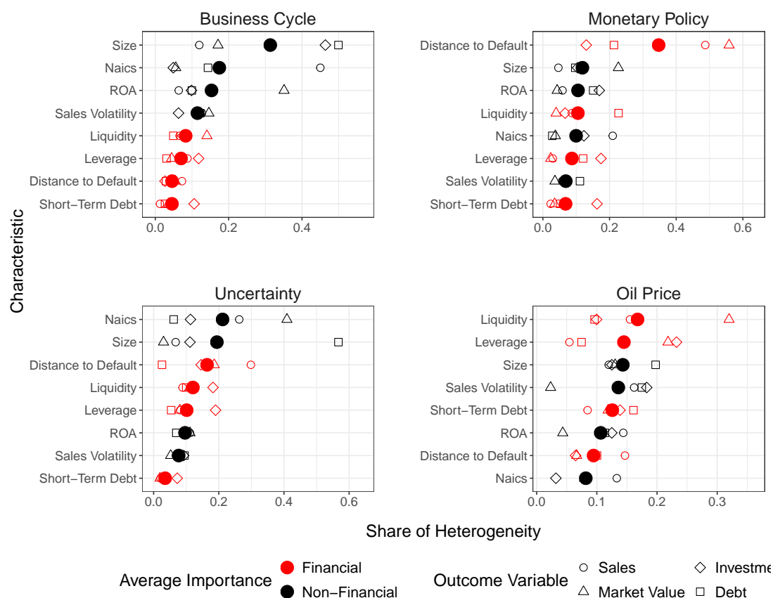
Figure 3: Characteristics importance for heterogeneity
