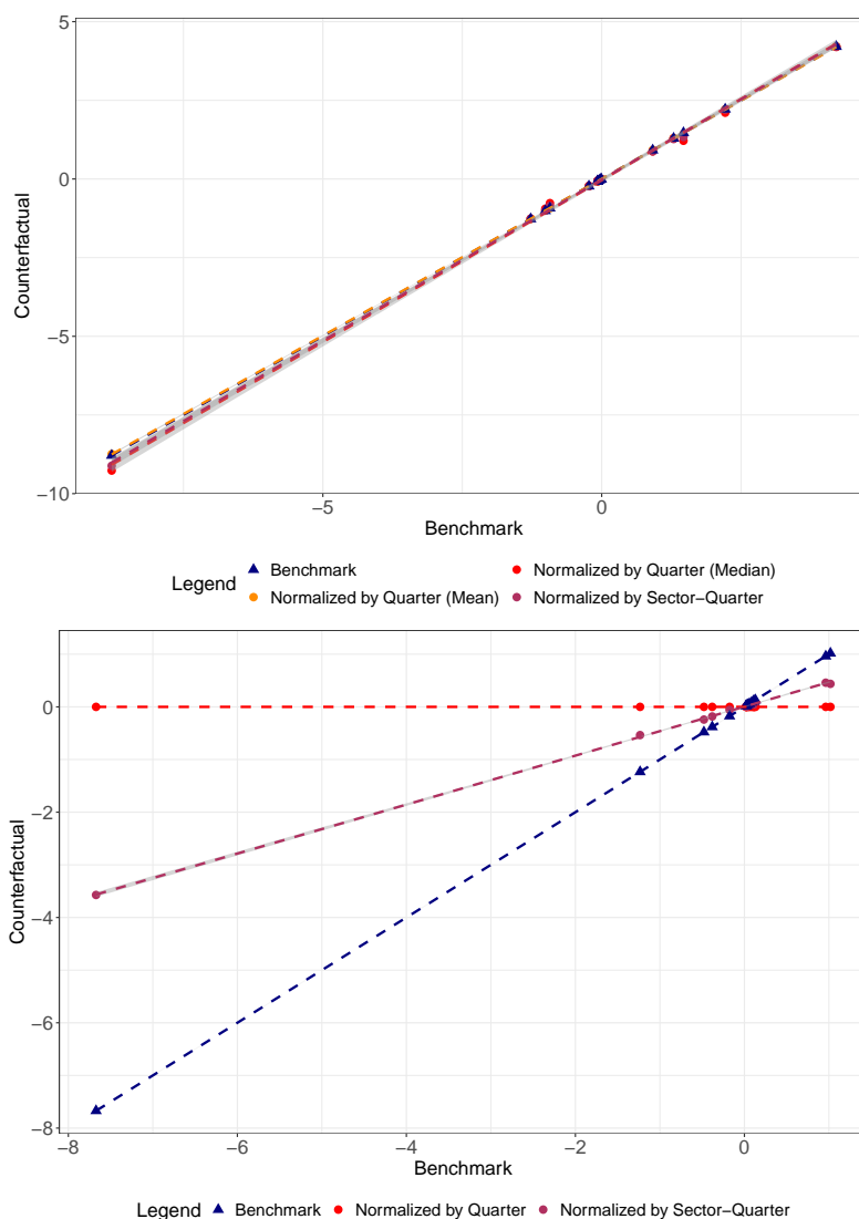
Figure 20: Within and across sector heterogeneity
